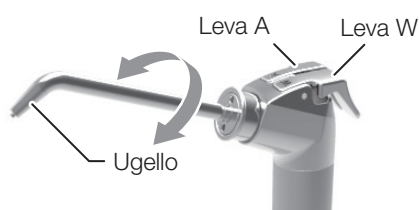
Siringa SYR-20 3WAY
